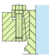
Shrink disk
