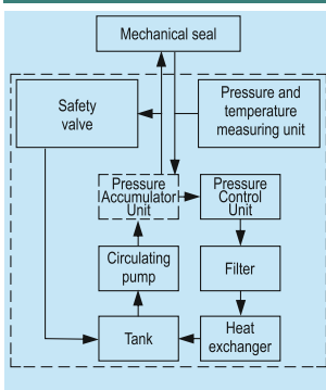
Installation and operating diagram for a BFS system.
