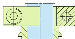
Clamping ring
